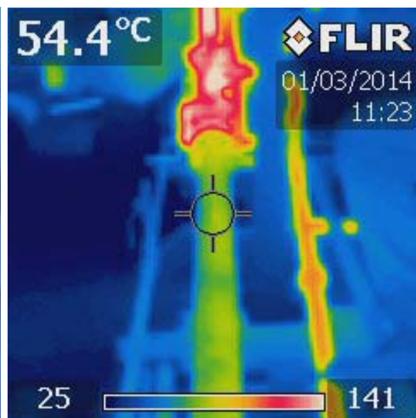
Hot Pipe Coating Insulation: 54 C
